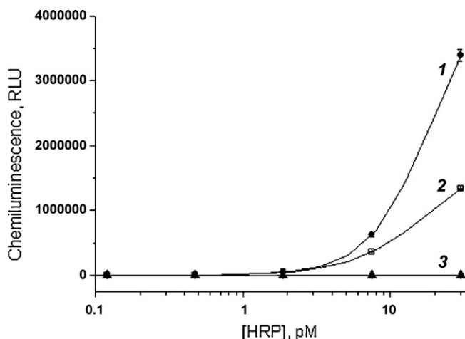
Fig. 4. Effect of HRP-C concentration on light output from luminol/ \text{H}_2\text{O}_2 substrates in the presence of SPTZ and MORP evaluated under following conditions: (1) [luminol]=0.17 mM; [ \text{H}_2\text{O}_2 ]=1.75 mM; [SPTZ]=2.1 mM; [MORP]=8.75 mM; 80 mM Tris buffer, pH 8.3, (2) [luminol]=0.75 mM; [ \text{H}_2\text{O}_2 ]=0.5 mM; [SPTZ]=1.0 mM; [MORP]=1.0 mM; 50 mM Tris buffer, pH 8.3, and (3) [luminol]=5 mM, [ \text{H}_2\text{O}_2 ]=4.0 mM; [SPTZ]=1.5 mM; [MORP]=1.5 mM; 125 mM Tris, pH 9.0. Chemiluminescence intensity was recorded 7.5 min after the start of the reaction. Each point represents the mean of triplicates. Vertical bars indicate \pm S.D. about the mean.
